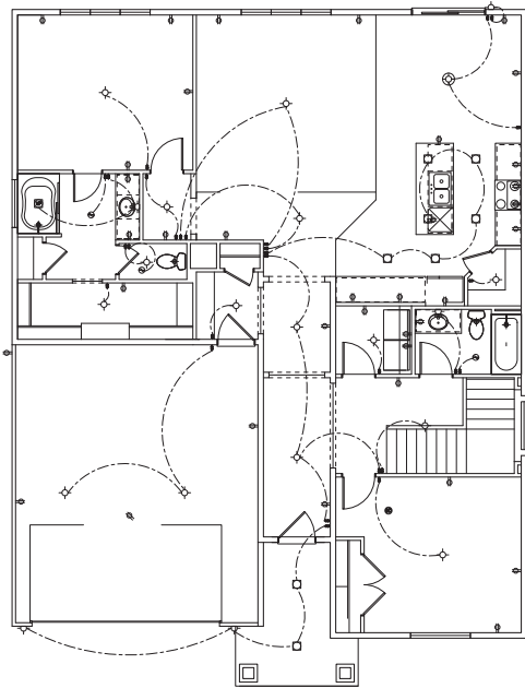
Main Level Electrical Plan
